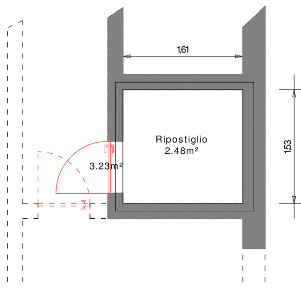
PIANO INTERRATO sub 48
